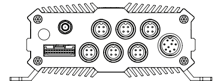
BACK VIEW WITH COVER REMOVED
