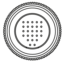
SECTION A-A PIN FACING 25-PIN THREADED PLUG - MALE
